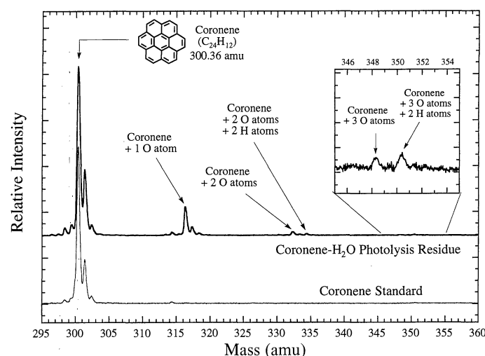
Fig. 1 (left). The \mu L^2MS spectrum of coronene ( C_{24}H_{12} ) compared with that of a residue from a photolyzed coronene- H_2O ice ( H_2O/PAH > 800 ). The peaks at 316, 332, and 348 amu correspond to the addition of one to three O atoms, respectively, likely in the form of ketones or hydroxyl side groups (or both). Elevated peaks at 334 and 350 amu (inset) indicate the addition of two H atoms to the doubly and triply oxygenated species. Fig. 2 (right). The \mu L^2MS spectrum of benzo[ghi]perylene ( C_{22}H_{12} ) compared with that of a
