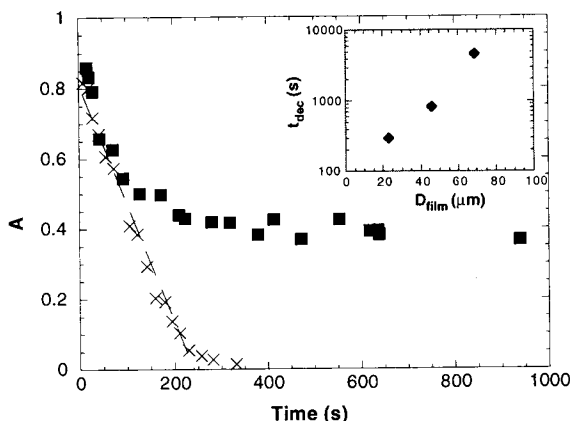
Fig. 3. The optical density A(t) of defects at time t after the quench from isotropic to cholesteric phase in a sample of thickness D_{\text{film}} = 23 \mu\text{m} (crosses: pure cholesteric; squares: cholesteric with inclusions). (Inset) The time constant t_{\text{dec}} in the linear regime A(t) = 1 - t/t_{\text{dec}} plotted as a function of D_{\text{film}} .
