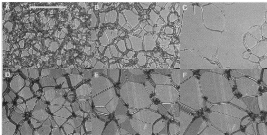
Fig. 2. (Upper row) Coarsening of the oily streak network in a pure cholesteric film with p = 7 \mu\text{m} and D_{\text{film}} = 40 \mu\text{m} [at times (A) t = 15 , (B) t = 30 s, and (C) t = 75 s after the quench] and in the same film with added colloidal inclusions [(D) t = 1 min, (E) t = 4 min, and (F) t = 7 min after the quench]. Imaging was performed with crossed polarizers; bar, 250 \mu\text{m} .
