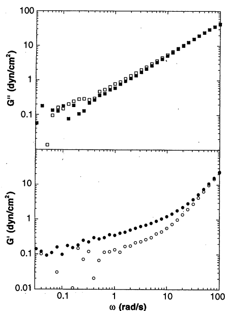
Fig. 4. Loss modulus ( G'' , squares) and storage modulus ( G' , circles) in the presheared cholesteric samples. The empty and filled symbols correspond to a sample without and with inclusions, respectively.
