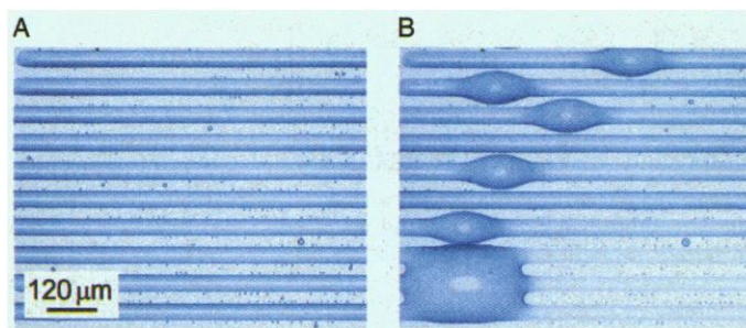
Fig. 1. Microchannels of water as observed by optical microscopy. (A) Low-coverage regime. The channels have a constant cross section and a small contact angle. (B) High-coverage regime. The channels developed a single bulge as soon as the contact angle exceeded a certain characteristic value. If two bulges of two neighboring channels are in close proximity, they may merge with each other (see the larger structure in the lower left corner).
