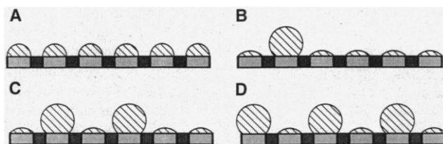
Fig. 3. Possible droplet patterns on a linear chain of circular domains. Because of the Laplace equation, all droplets must have the same mean curvature, which implies that the small and the large droplet must form a complete sphere when pasted together along their flat contact areas. All droplet patterns, such as (C) and (D), that contain more than one large droplet are unstable and must decay into the homogeneous pattern (A) or into the heterogeneous pattern (B) with only one large droplet.
