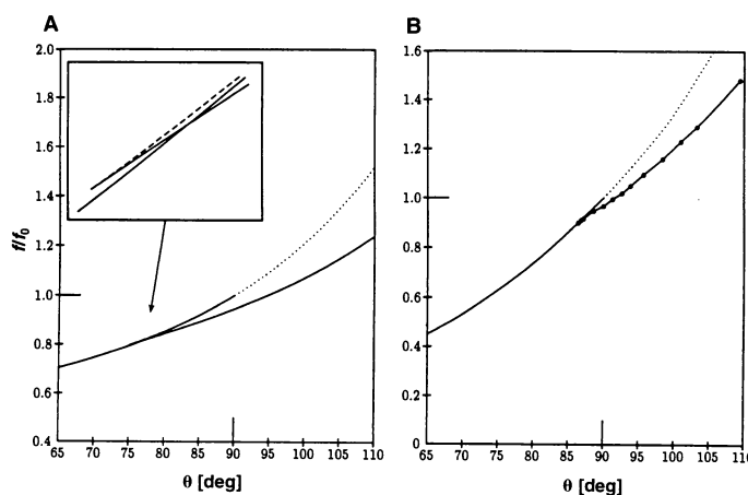
Fig. 4. Bifurcation of channel states: free energy ff_0 as a function of the angle \theta . For the homogeneous channel, \theta is the actual contact angle; for the bulge state, \theta is the contact angle of the homogeneous channel, which has the same volume as the bulge state. The scale f_0 is the free energy of the homogeneous channel with \theta = 90^\circ . At \theta = \theta_* , the homogeneous state becomes metastable, and the state with a single bulge becomes the state of lowest free energy. At \theta = \theta_{max} = 90^\circ , the homogeneous channel becomes unstable. The dotted line in (A) and (B) represents this unstable state. The dashed line in the inset of (A) corresponds to another unstable state. (A) and (B) were obtained from the approximation in Fig. 3 and from numerical minimization, respectively.
