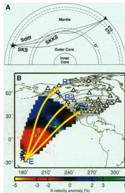
Fig. 1. (A) Schematic representation of the wavepaths of SKS , SKKS , and Sdiff . (B) Earthquakes (stars), stations (triangles), and projections of the raypaths (gray solid lines) used in the forward modeling presented in this study. We used 31 events from 1962 to 1998. Our data set consists of our own measurements and data from (18). Note the good coverage of the central Pacific. Paths E1-R1, E2-R2, and E3-R3 correspond to the depth cross sections presented in Fig. 5. Color contours correspond to our preferred S -velocity model for the region covered by our data set at 2700-km depth. Symbols S and F point to the slow and fast domains discussed in the text and also presented in the depth cross sections of Fig. 5.
