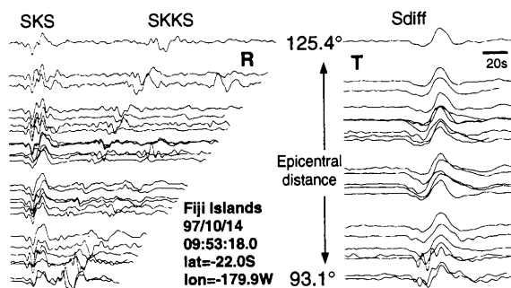
Fig. 2. Examples of records for event 97/10/14 and stations in North America. The azimuths considered are between 0^\circ and 60^\circ . R (radial) components are displayed on the left, and T (transverse) components are on the right. The similarity of the waveforms between SKS and S, and from one station to another, yields differential measurements with low scatter (Fig. 3A). We did not select data by narrow azimuthal corridors as in the study described in the text.
