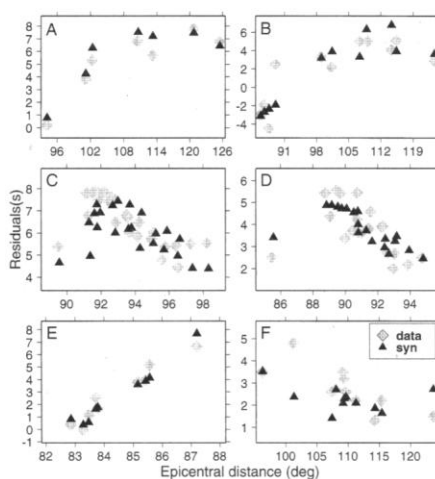
Fig. 3. Examples of observed variations of differential travel time residuals for S - SKS as a function of epicentral distance (gray diamonds) along with synthetic predictions (black triangles) computed for our preferred 3D model. (A and B) Data and predicted residuals for events 97/10/14 and 98/03/29, respectively, and azimuths between 40^\circ and 50^\circ . S penetrates into the slow velocity region (see Fig. 4) as distance increases, and S - SKS residuals correspondingly increase. (C and D) Same as (A) and (B) for events 92/06/25 and 92/07/11, respectively. The trend is opposite that observed in (A) and requires a fast region where the S-velocity anomaly reaches +5% (see Fig. 5). (E) S - SKS residuals for fixed-station COR and several Fiji-Tonga-Kermadec Islands events, and azimuths between 35^\circ and 37^\circ . (F) SKKS - SKS residuals for event 98/03/29, and azimuths between 40^\circ and 60^\circ .
