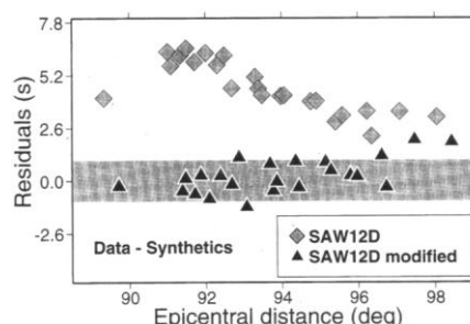
Fig. 4. Examples of differences between observed and predicted S - SKS residuals for model SAW12D and for our preferred 3D model. Residuals are for event 92/06/25 (E in Fig. 1B). By amplifying the magnitude of heterogeneity in regions S and F (see Figs. 1B and 5), it is possible to improve the fit significantly.
