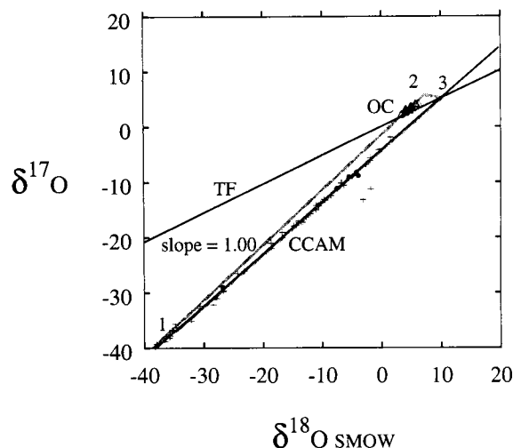
Fig. 1. Three-isotope plot for oxygen showing the positions of the TF line, the CCAM line, as represented by data in (9) (crosses) for the Allende CV carbonaceous chondrite, and the field for OCs, as represented by data in (37) (triangles). Closed circles are analyses of a type B1 CAI from Allende sample 3576 reported in (17). The corners of the gray triangle labeled 1, 2, and 3 represent the minimum number of distinct oxygen reservoirs in the early solar nebula if the CCAM line represents mixing between ^{16}\text{O} -rich material (but not pure ^{16}\text{O} , in the direction of 1) and ^{16}\text{O} -poor material (4) without modification by physicochemical mass-dependent fractionation. The isotopic compositions of protoplanetary minerals would fall within the region bounded by the gray triangle if the CCAM is attributable to mixing without fractionation. The two CAI data points to the right of the CCAM are from a FUN inclusion (FUN refers to fractionation and unidentified nuclear effects) (9).
