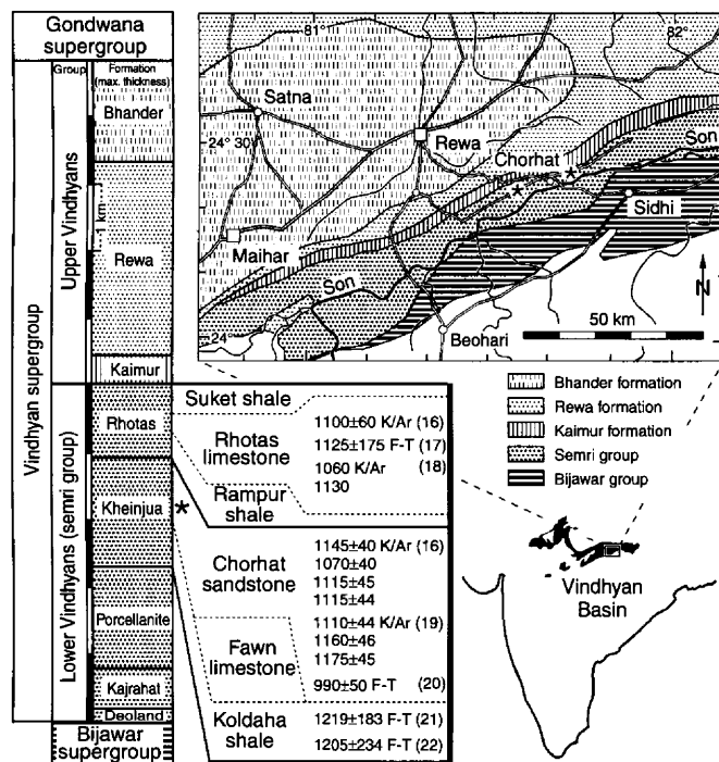
Fig. 1 (left). The Vindhyan Supergroup, central India, with stratigraphic context, location of metazoan burrows (stars), and published ages with references. Ages are millions of years ago and calculated by the potassium/argon method (K/Ar) or by fission tracks (F-T). Fig. 2 (right). Worm burrows from the Mesoproterozoic Chorhat Sandstone of central India support the claim of molecular biologists that triploblastic metazoans existed twice as long ago as the assumed Cambrian evolutionary explosion of modern animal phyla. A remnant of the original sand veneer cover (arrow) shows that the burrows are not modern artifacts (Yale specimen YPM 37665). (Photograph by W. Sacco)
