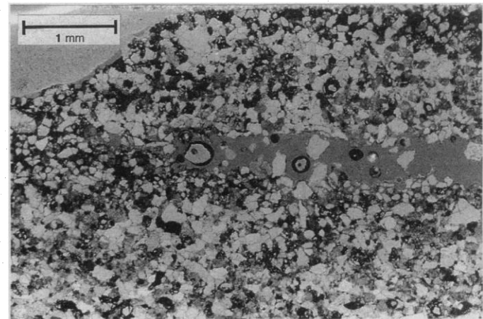
we assume that the wormlike maker was an undermat miner [part of the burrow that is still covered by the original sand veneer is indicated by the arrow (see Fig. 2)]. Panels 1 to 4 show further examples, which were drawn from casts and field photographs, and insets A to D show different blocks of the bed. Fig. 5 (bottom right). A thin section of the trace-bearing bed (Fig. 4, inset A). The grains are less closely packed (and have a larger amount of dark matrix) in the upper 2 mm, where they were microbially bound. The section broke at about the level of the burrows during preparation.
