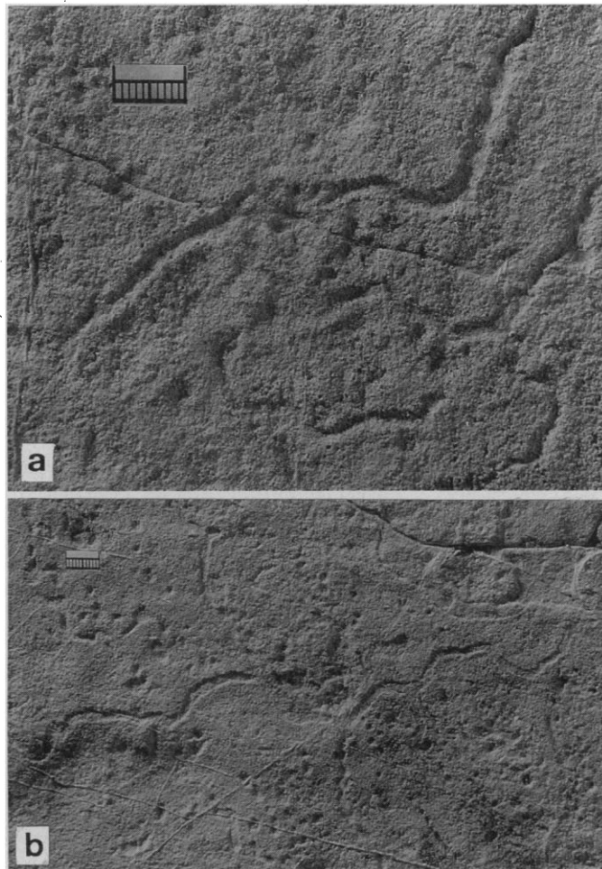
Fig. 3 (left). Chhorhat worm burrows on a weathered top surface. The patterns are unlike syneresis cracks, and (a) elevated rims provide evidence that these burrows are not modern artifacts. (b) Elevated crack fillings suggest the thickness of veneer that has been weathered away (casts in Tübingen collection, GPIT 1847/1-2). (Photograph by W. Gerber) Fig. 4 (top right). The burrows [block diagram of Fig. 1 drawn from the outcrop situation and the cast in the Tübingen collection (GPIT 1847/3)] become visible only after the top millimeter of the sandstone bed has been weathered away. Fresh surfaces lack such burrows except for less distinct collapse structures. Therefore,
