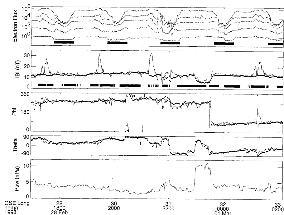
Fig. 2. Time series of electron and magnetic field measurements obtained when the moon was in the solar wind. The series spans five consecutive orbits passing over selenographic longitudes near 0^\circ and 180^\circ ; successive orbits are separated by \sim 1^\circ in longitude at the equator. Electron flux ( \text{cm}^{-2} \text{s}^{-1} \text{sr}^{-1} \text{eV}^{-1} ) is shown at five energies (top to bottom): 40, 140, 340, 800, and 2950 eV. Solid bars below the 2950-eV trace indicate times when the spacecraft was in the moon's optical shadow. The magnetic field amplitude and direction in selenocentric solar ecliptic coordinates are shown as solid lines in the next three panels. Measurements of the solar wind magnetic field by the WIND spacecraft, located \sim 1.2 million km upstream of the moon, are time-shifted to allow for the \sim 50 -min solar wind travel time from WIND to LP and superimposed as solid dots over the LP observations. Solid bars below the magnetic field amplitude indicate times when LP is magnetically connected to the lunar surface. (Bottom) The solar wind dynamic pressure ( P_{sw} = \rho v^2 , where \rho and v are the solar wind mass density and flow velocity, respectively) as measured by WIND and time-shifted to LP's position. The moon's geocentric solar ecliptic (GSE) longitude is indicated along the time axis.
