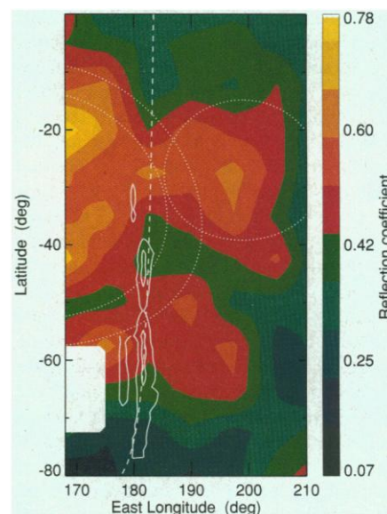
Fig. 1. The electron reflection coefficient, a measure of crustal magnetic fields (16), is mapped over a region of the lunar far side in a cylindrical equidistant projection. These data were obtained during the first four passes (February to May 1998) through the geomagnetic tail (but outside of the current sheet), where the magnetic field and electron flux are steady. Reflection coefficients from > 1000 three-dimensional samples, each with a spatial resolution of \sim 4 km, are averaged into 7.5^\circ by 7.5^\circ bins ( \sim 200 km on a side); then smooth contours are drawn around the binned data and color coded. The antipodal zones of the Imbrium and Serenitatis ringed impact basins are indicated by the dotted circles. The two circles for Imbrium correspond to its main rim \sim 1200 km in diameter and a partial rim at 1500 km (9). For Serenitatis the single rim is \sim 740 km in diameter. The solid contours show where the spacecraft (at an altitude of \sim 100 km) passed through large amplifications of the solar wind magnetic field that form as the solar wind is shocked and deflected by the crustal magnetic field. The contours are at 20 and 27 nT, and the ambient field is nearly constant at \sim 10 nT. The orbit track corresponding to the second enhancement in Fig. 2 is shown by the dashed line.
