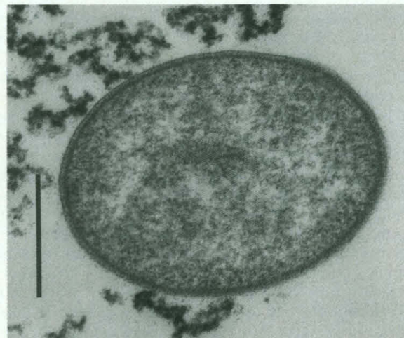
Fig. 3. Transmission electron photograph of a hyperthermophilic archaeon isolated from North Gorda event plume water (16). Hyperthermophiles were not found in background ocean water. Scale bar = 0.4 \mu\text{m} .
