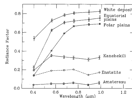
Fig. 4. Spectral reflectances on Io as seen with six SSI color filters. The bulk of Io's surface (white deposits and plains units) has a flat spectrum from 0.75 to 1.0 \mu\text{m} , but the dark features covering a few percent of the surface (such as Kanehekili and Amaterasu, shown here) are relatively dark in the 0.89- \mu\text{m} bandpass. The ultraviolet absorption at Kanehekili (drop in reflectance at 0.4 \mu\text{m} ) is typical of all but the darkest features and is evidence for the presence of sulfurous materials in addition to silicates (34). Also shown is the spectrum for an enstatite (orthopyroxene) with 5% FeO (35) convolved to the SSI bandpasses and vertically scaled to place it between the Kanehekili and Amaterasu spectra.
