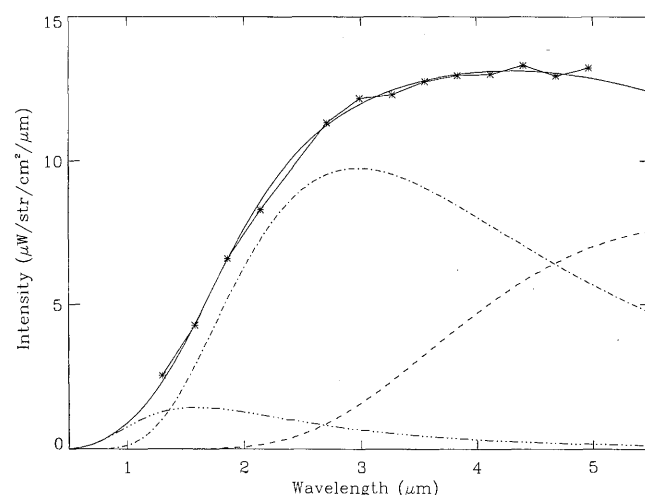
Fig. 3. Three-temperature fit to NIMS spectrum of Pillan and Pele hot spots in orbit C9. Three blackbody curves are shown: dashed curve for 544\text{-km}^2 area at 475 K, dash-dot curve for 17.6\text{-km}^2 area at 975 K, and dash-dot-dot curve for 0.11\text{-km}^2 area at 1825 K. The smooth solid curve is the sum of the three blackbody curves, and the asterisks mark the NIMS data points.
