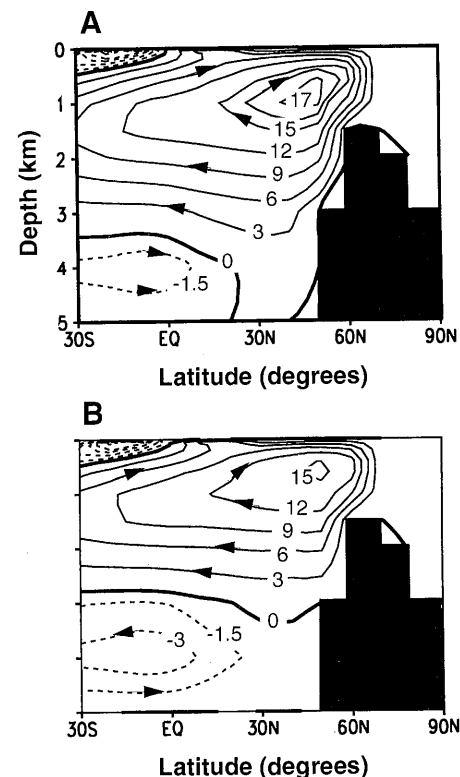
Fig. 4. Meridional transport stream function (in \text{Sv} = 10^6 \text{ m}^3/\text{s} ) in the Atlantic for the control run (A) and for simulation AOV (B). Black boxes indicate ocean topography.
