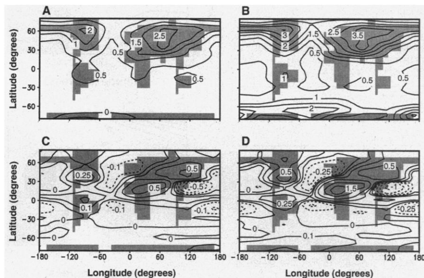
Fig. 2. Differences in near-surface air temperature (in ^\circ\text{C} ) during boreal summer between two of our four mid-Holocene simulations and the present-day control run. ( A ) Simulation A minus control. ( B ) Simulation AOV minus control. ( C and D ) are the same as ( A ) and ( B ), respectively, but for precipitation (in mm/day). Dashed lines indicate negative differences.
