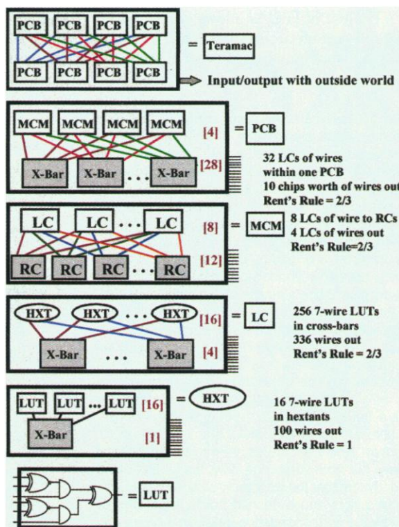
Fig. 2. The logical map of Teramac.
