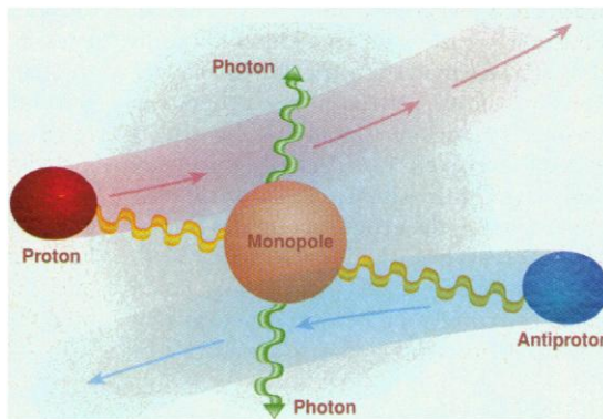
Little big bang. If colliding protons spawned a monopole, a pair of high-energy photons (green) might reveal it.
