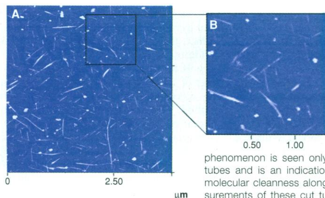
Fig. 2. (A and B) Tapping mode AFM images of cut fullerene nanotubes (pipes) electrodeposited from a stable colloidal suspension onto HOPG. Note the tendency of tubes to align 120° to one another, presumably in registry with the underlying graphite lattice. This phenomenon is seen only with well-purified fullerene tubes and is an indication of a very high degree of molecular cleanliness along the tube sides. AFM measurements of these cut tubes show that roughly half
