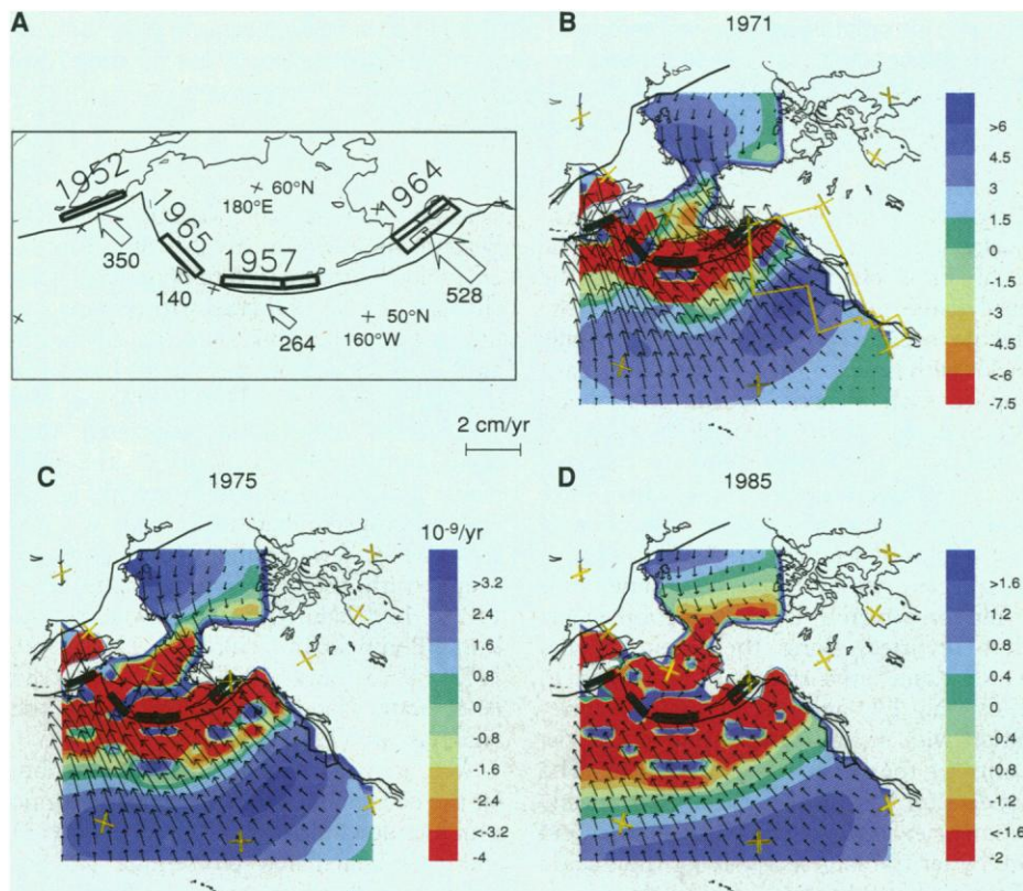
Fig. 1. (A) Rupture areas of major subduction events along the Aleutian arc and Kamchatka trench from 1952 to 1965. Arrows give the direction of slip associated with each of the four events considered, with length proportional to total seismic moment. Numerals adjacent to these arrows specify the seismic moment in units of 10^{20} N·m (30). (B through D) Net postseismic velocity and dilatational strain rate \dot{\epsilon}_{EE} + \dot{\epsilon}_{NN} (E, east; N, north) over the northern Pacific and eastern Arctic basins driven by combined subduction events projected onto a sphere centered on 50^\circ N, 155^\circ W as evaluated at three different times. Deformation is evaluated at Earth's surface. Heavy lines denote the fault planes used to model the subduction events. Locally large velocities near the rupture zones have been truncated at a maximum of 5 \text{ cm year}^{-1} for visual simplicity.
