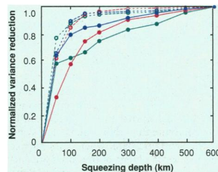
Fig. 3. Normalized variance reduction versus squeezing depth Z_s for inversions of observed (solid curves) and synthetic (dashed curves) data. Curves for P , S_{\text{slow}} , and S_{\text{fast}} are shown in green, blue, and red, respectively.
