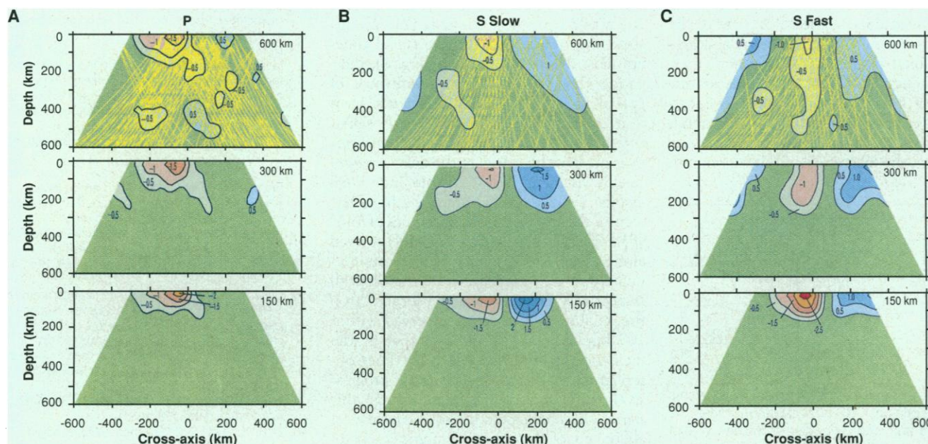
Fig. 2. Results of tomographic imaging contoured in percent deviation from a radial Earth model (9); the delay time observations do not constrain absolute velocities, so only relative variations are meaningful. Contour interval is 0.5%; zero contour not shown. Cross-axis direction is positive to the east. (A) P image; (B) S_{\text{slow}} image; (C) S_{\text{fast}} image. Percent deviations more negative
