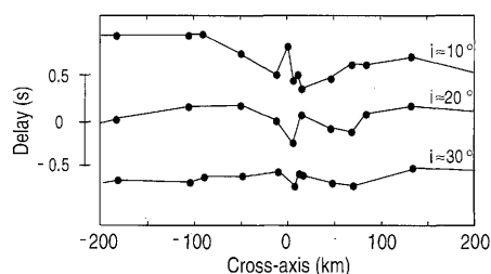
Fig. 4. Delay times of P waves from three events along the primary OBS array (shifted vertically for clarity). At near-vertical angles of incidence (that is, small values of the incidence angle i ), the gradual decrease in the delays toward the rise axis is consistent with a near-vertical alignment of the crystallographic a axis of upper-mantle olivine crystals in an upwelling region with a half-width of about 100 km.
