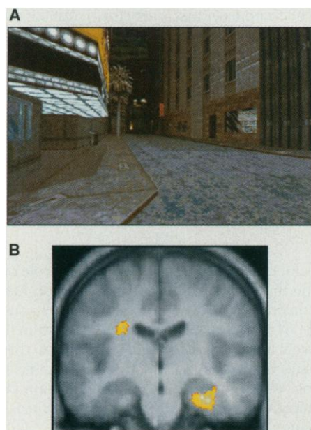
Fig. 1. (A) Example of view from inside the virtual town. (B) The comparison between successful navigation (nav1 and nav2) compared to following a trail of arrows. PET data are superimposed onto the averaged MRI of the 10 subjects at the voxel of peak activation in the right hippocampus displayed in the coronal plane. The color scale of the activation pertains to the significance level of the z scores with the peak of the activation in white. Coordinates in stereotactic space (x,y,z, respectively) and z scores of the activations are: right hippocampus (30, -16, -22; z = 3.74) and left tail of caudate (-28, -16, 28; z = 3.05). Other areas activated in this comparison but not displayed on this plane were: left occipital area 18 (-24, -102, -2; z = 3.50) and left superior frontal gyrus (-22, 52, 22; z = 3.65). The comparison between successful versus lost trials showed the following activations: right hippocampus (30, -20, -16; z = 3.61); left hippocampus (-16, -26, -6; z = 4.10); left superior temporal gyrus (-54, -30, 14; z = 3.86); left inferior temporal gyrus (-52, -50, -12; z = 5.23); left inferior frontal gyrus (-46, 22, 6; z = 4.59); and right thalamus (6, -6, 12; z = 4.25).
