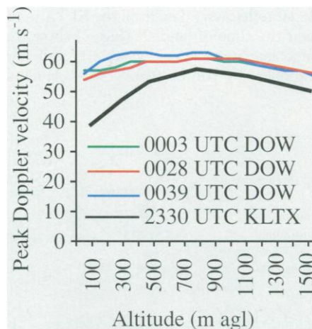
Fig. 6. Altitude dependence of peak wind speeds as observed by DOW and National Weather Service KLTX radars. DOW-measured peak speeds at 100 m agl are nearly as high as those at 1000 m agl as a result of momentum transport in the rolls and agree closely with surface peak wind observations. KLTX-measured peak speeds are smaller at low altitude because of poorer resolution and possibly because of longer overland trajectories.
