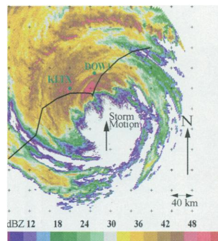
Fig. 2. Large-scale radar reflectivity (dBZ) structure of the eye and surrounding rain bands in hurricane Fran as it made landfall on the North Carolina coast at 2327 UTC 05 September 1996, as measured by the KLTX National Weather Service WSR-88D radar. Rain bands surrounding the large eye and structures within the rain bands, particularly to the north and northwest of the eye, contain features with \sim 10 -km scale. Scan is at 0.5^\circ elevation (17).
