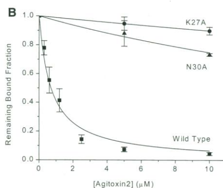
Fig. 3. Binding affinity of wild-type and mutant agitoxin2 to the mutant KcsA K + channel. (A) Quantity of radiolabeled agitoxin2 bound to 0.3 \mu l of cobalt resin saturated with the mutant KcsA K + channel as a function of the radiolabeled agitoxin2 concentration (17). Each point is the mean \pm SEM of four measurements, except for the 0.03 \mu M and 1.5 \mu M concentrations, which are the mean \pm range of mean of two measurements. The curve corresponds to equation: bound agitoxin2 = A \times \{1 + K_D/[\text{agitoxin2}]\}^{-1} , with equilibrium dissociation constant K_D = 0.62 \mu M and resin capacity A = 16 pmol. (B) Remaining bound fraction of radiolabeled wild-type toxin as a function of the concentration of unlabeled wild-type toxin or mutant toxins K27A or N30A (17). Each point is mean \pm SEM of four measurements for wild-type agitoxin2 (squares) or mean \pm range of mean of two measurements for K27A (circles) and N30A (triangles) agitoxin2 mutants. The curves correspond to equation: remaining bound fraction = \{1 + K_{Dhot}/[\text{agitoxin2}_{hot}] \times \{1 + (K_{Dhot}/[\text{agitoxin2}_{hot}]) \times (1 + [\text{agitoxin2}_{cold}]/K_{Dcold})\}^{-1}\}^{-1} with labeled toxin concentration [\text{agitoxin2}_{hot}] = 0.06 \mu M, wild-type toxin K_{Dhot} = 0.62 \mu M, and competing toxin dissociation constant K_{Dcold} = 0.62 \mu M (wild type), 81 \mu M (K27A), and 27 \mu M (N30A). (C) CPK model of the interaction surface of agitoxin2 (18). Side chains of functionally important amino acids are in red (4). This figure was prepared with the program GRASP (19).
