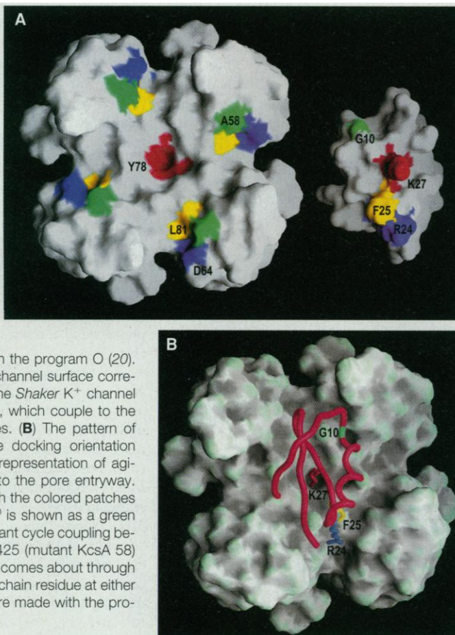
Fig. 4. Docking of agitoxin2 onto the KcsA K + channel. (A) Molecular surface of the pore entryway of the KcsA K + channel (left) and agitoxin2 (right). The colors indicate locations of interacting residues on the toxin and channel surfaces as determined by thermodynamic mutant cycle analysis of the Shaker K + channel-agitoxin2 interaction (4, 8). The three pore mutations of the KcsA K + channel used in this study (Q58A, T61S, and R64D) were introduced into the channel model with the program O (20). Indicated residues on the channel surface correspond to the positions of the Shaker K + channel equivalent residues (Fig. 1), which couple to the indicated agitoxin2 residues. (B) The pattern of colors in (A) suggests the docking orientation shown by the main chain representation of agitoxin2 placed manually onto the pore entryway. The side chain colors match the colored patches in (A). The position of Gly 10 is shown as a green band on agitoxin2. The mutant cycle coupling between residues at Shaker 425 (mutant KcsA 58) and residue 10 of agitoxin2 comes about through substitution of a bulky side chain residue at either position (4, 7). Pictures were made with the program GRASP (19).
