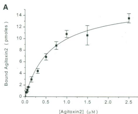
Fig. 3. Binding affinity of wild-type and mutant agitoxin2 to the mutant KcsA K + channel. (A) Quantity of radiolabeled agitoxin2 bound to 0.3 \mu l of cobalt resin saturated with the mutant KcsA K + channel as a function of the radiolabeled agitoxin2 concentration (17). Each point is the mean \pm SEM of four measurements, except for the 0.03 \mu M and 1.5 \mu M concentrations, which are the mean \pm range of mean of two measurements. The curve corresponds to equation: bound agitoxin2 = A \times \{1 + K_D/[\text{agitoxin2}]\}^{-1} , with equilibrium dissociation constant K_D = 0.62 \mu M and resin capacity A = 16 pmol. (B) Remaining bound fraction of radiolabeled wild-type toxin as a function of the concentration of unlabeled wild-type toxin or mutant toxins K27A or N30A (17). Each point is mean \pm SEM of four measurements for wild-type agitoxin2 (squares) or mean \pm range of mean of two measurements for K27A (circles) and N30A (triangles) agitoxin2 mutants. The curves correspond to equation: remaining bound fraction = \{1 + K_{Dhot}/[\text{agitoxin2}_{hot}] \times \{1 + (K_{Dhot}/[\text{agitoxin2}_{hot}]) \times (1 + [\text{agitoxin2}_{cold}]/K_{Dcold})\}^{-1}\}^{-1} with labeled toxin concentration [\text{agitoxin2}_{hot}] = 0.06 \mu M, wild-type toxin K_{Dhot} = 0.62 \mu M, and competing toxin dissociation constant K_{Dcold} = 0.62 \mu M (wild type), 81 \mu M (K27A), and 27 \mu M (N30A). (C) CPK model of the interaction surface of agitoxin2 (18). Side chains of functionally important amino acids are in red (4). This figure was prepared with the program GRASP (19).
