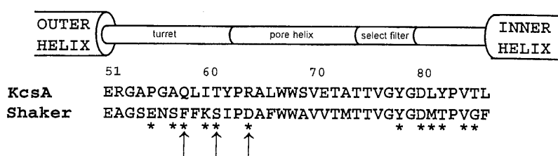
Fig. 1. Sequence alignment of the KcsA and Shaker K^+ channel pore regions. The numbering for KcsA is above the sequences. Structural elements are indicated (5). Asterisks, several Shaker K^+ channel amino acid locations where mutations influence agitoxin2 binding (4, 8, 9); arrows, the three KcsA K^+ channel amino acids mutated in this study. The sequences are KcsA, S. lividans , accession number (acc) PIR S60172; and Shaker, Drosophila melanogaster , acc PIR S00479.
