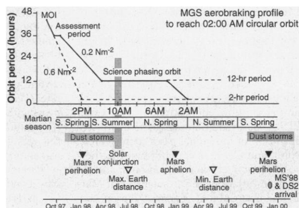
Fig. 1. Mission profile showing the phasing of aerobraking orbits, assessment orbits, science-phasing orbits, and circular orbits. Orbit period in hours is plotted against time and temporal events, including solar conjunction, nominal dust storm periods, Earth-Mars-sun distances, martian seasons, and arrival of Mars Surveyor '98 (MS98) (3) at Mars. The slope in the aerobraking periods corresponds to the average pressure exerted on the solar panels 0.6 \text{ N m}^{-2} during the first aerobraking period and 0.2 \text{ N m}^{-2} during the second and third periods. The orientation of the MGS orbit relative to the sun at noon is indicated by the times shown on the horizontal axis. MOI, Mars Orbit Insertion; S, southern; N, northern.
