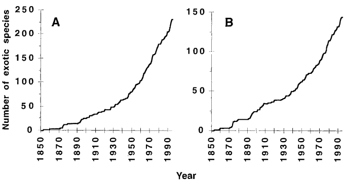
Fig. 1. Cumulative number of exotic species established in the San Francisco Estuary: (A) raw data; (B) modified data. A time series analysis conducted by C. Parmesan [Box-Jenkins methodology (19) on RATS (Regression Analysis of Time Series) software, version 4.0 (Estima); final models used only terms that contributed significantly at P < 0.05 and had uncorrelated residuals by Durbin-Watson and Ljung-Box Q statistics] showed a significant increase in the number of invasions over time (linear regression on raw and modified data separately, trend terms significant at P < 0.001 ). Trend = (time) 2 models explained 5% and 2% more of the variation than did trend = time models for raw and modified data sets, respectively (final models: R^2_{\text{raw}} = 0.34 , R^2_{\text{modified}} = 0.21 ). Additional lag terms on time were unnecessary (and when forced into the models were not significant at P > 0.50 for both data sets), indicating that invasion events are independent between years. A better fit of trend = (time) 2 models indicates that the rate of invasions, as well as the absolute number, increases with time.
