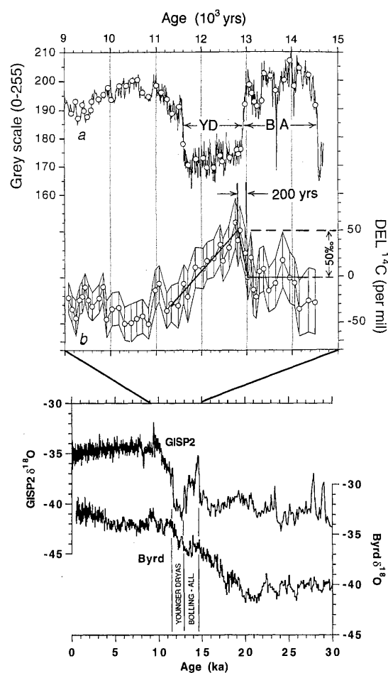
Fig. 4. Evidence in support of the existence of a bipolar seesaw in thermohaline circulation during the period of deglaciation. In the lower panel is shown the correlation between the stable isotope records for ice cores from Greenland (GISP2) and Antarctica (BYRD). This correlation is based on measurements of ^{18}\text{O}/^{16}\text{O} ratios of \text{O}_2 trapped in bubbles in the ice (37). The time scale is based on annual layer counts in the GISP2 core (55). As can be seen, an antiphasing exists between the ^{18}\text{O} increases (that is, warmings) at the two locales. That this antiphasing is related to changes in the rate of deep sea ventilation is dramatically demonstrated by the record of atmosphere-upper ocean ^{14}\text{C}/^{12}\text{C} ratio reconstructed from radiocarbon measurements on foraminifera from varved marine sediments, in the Cariaco Trench (38). As shown in the upper panel, during the first 200 years of the Younger Dryas (Y.D.) cold event (marked in Cariaco sediments by a prominent color change), newly produced radiocarbon atoms were backlogged in the atmosphere-upper ocean reservoir, reflecting a shutdown of deep ventilation (that is, the Conveyor). During the remainder of the Y.D., this radiocarbon excess was gradually removed by downward mixing into the large deep sea reservoir. Because the cold climate generated by the shutdown of Conveyor circulation was not ameliorated by this renewed ventilation, the burial of ^{14}\text{C} more likely occurred in the Southern Ocean than in the northern Atlantic (39).
