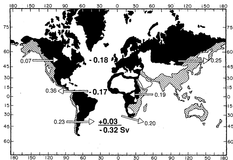
Fig. 2. Hydrologic budget (12) for the Atlantic Ocean and its continental drainage basin (shown in black). The lands shown by shading drain to the Pacific and Indian oceans. The white areas are deserts from which no drainage occurs. Westerly winds in the Northern Hemisphere transport more water vapor across Asia than enters across the American cordillera. Easterly winds carry more water vapor out across Central America than enters across Africa. The light numbers give the inputs and losses of water vapor in three latitude zones: north temperate, tropical, and south temperate. The bold numbers give the net loss from each of these zones and for the Atlantic as a whole. The net result based on the Oort's (12) global humidity and wind data set is a loss of 0.32 Sv (that is, a bit over the flow of the Amazon River) from the Atlantic to the Pacific. Were this flux not compensated by an exchange of more salty Atlantic waters for less salty Pacific waters, the salinity of the entire Atlantic would rise about 1 gram per liter per millennium.
