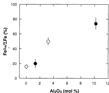
Fig. 1. Variation of \text{Fe}^{3+}/\Sigma\text{Fe} with Al content of (Mg,Fe)SiO _3 perovskite. Open circles are from previously reported multianvil experiments (16) and solid circles are from São Luiz diamond inclusions (present work). Iron compositions [expressed as \text{Fe}/(\text{Fe} + \text{Mg}) ] of the (Mg,Fe,Al)(Si,Al) \text{O}_3 and perovskite phases range between 5 and 9%.
