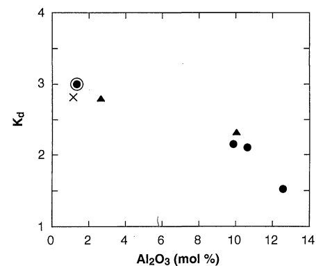
Fig. 2. Variation of Fe-Mg partition coefficient between (Mg,Fe,Al)(Si,Al) \text{O}_3 and (Mg,Fe)O inclusions [ K_d = (X_{\text{Fe}}^{\text{mw}}/X_{\text{Mg}}^{\text{mw}})/(X_{\text{Fe}}^{\text{pv}}/X_{\text{Mg}}^{\text{pv}}) ] with Al content. Solid circles are from São Luiz electron microprobe data from (24), where the outlined circle indicates the pair examined by Mössbauer spectroscopy in the present study (BZ251). Solid triangles are from São Luiz electron microprobe data of (2). The cross refers to the only known (Mg,Fe,Al)(Si,Al) \text{O}_3 -(Mg,Fe)O inclusion pair not from São Luiz (27).
