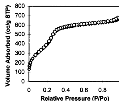
Fig. 5. Nitrogen adsorption isotherm data obtained on aligned calcined mesoporous silica synthesized through a liquid crystalline intermediate and polymerized with vapor phase HCl (method 1). The nitrogen adsorption and desorption isotherms are characteristic of mesoporous samples (47).
