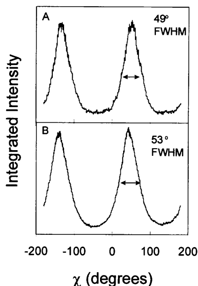
Fig. 4. Radial integrations over the width of the (100) hex diffraction peak (in Fig. 2) plotted as integrated x-ray scattering intensity versus radial position \chi for (A) the aligned polymerized hexagonal silica-surfactant composite and (B) aligned calcined hexagonal mesoporous silica. The data show Gaussian distributions of domain orientations with a 49^\circ FWHM for the aligned silica-surfactant composite in (A) and a 53^\circ FWHM for the aligned calcined mesoporous material in (B).
