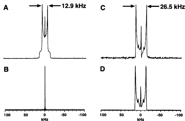
Fig. 1. In situ ^2\text{H} NMR spectra (A to C) and simulation (D) of a two-phase silicate-surfactant liquid crystal sample at pH = 12.5 made with \alpha -deuterated CTAB showing different stages of the thermal and magnetic field alignment process. (A) Powder pattern at 25°C, corresponding to an initially unaligned hexagonal liquid crystal with a random distribution of domain directors. (B) Isotropic spectrum of a silicate-surfactant mesophase at 90°C, above the anisotropic-to-isotropic transition temperature of the liquid crystalline phase. The single peak indicates rapid, isotropic motion of the surfactant molecules corresponding to a loss of hexagonal order. (C) After slow cooling from 90° to 25°C in the presence of an 11.7-T magnetic field, the hexagonal liquid crystal phase is restored. The altered intensity distribution in the spectrum compared with that observed in (A) indicates appreciable alignment of the liquid crystalline domains within the sample. (D) Simulated ^2\text{H} NMR spectrum generated assuming 80% of the CTA ^+ molecules are in hexagonal domains whose directors are oriented on average parallel to the applied field with a FWHM distribution of 55^\circ \pm 5^\circ , 15% of the CTA ^+ molecules are in randomly oriented hexagonal domains and 5% are rapidly mobile in the aqueous-rich phase.
