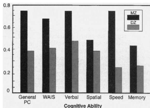
Fig. 2. Intraclass correlations for identical twins (MZ; black bars) and fraternal twins (DZ; gray bars) for general cognitive ability (PC and WAIS) and specific cognitive abilities.
