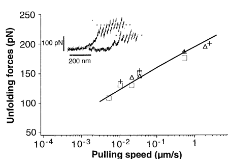
Fig. 5. The force required to unfold a domain is dependent on the pulling speed. The figure shows the average unfolding force measured while pulling segments of native titin at different speeds. The inset at upper left shows a typical experiment. A titin segment 500 nm long was pulled at a speed of 0.5 \mu\text{m/s} . The resulting force extension curve shows nine peaks averaging 190 pN. When the speed was reduced to 0.01 \mu\text{m/s} , the average force dropped to 130 pN. The graph shows the result of three different experiments ( \square , \Delta , and + ). A thousandfold reduction in the pulling rate reduced the average force required for unfolding by \sim 100 \text{ pN} . These data are well described by a Monte Carlo simulation of the unfolding of consecutive domains stretched at a constant speed (solid line). The Monte Carlo simulation was done as follows: The force generated by stretching the polypeptide chain is calculated with the WLC model shown in Fig. 3, using the parameters from these data (a persistence length of 0.4 \text{ nm} ; unfolding of a domain always lengthens the polypeptide by 28 \text{ nm} ). The probability of unfolding was calculated as P = \alpha \Delta t , where \Delta t is the polling interval and \alpha is the rate constant for unfolding given by \alpha = \alpha_0 \exp(F\Delta x/kT) (19), where \alpha_0 is the unfolding rate in the absence of an external force, F is the applied force, and \Delta x is the width of the unfolding potential. The simulation was done by stretching the polypeptide chain by a small amount, computing the resulting force with the WLC model, calculating the domain unfolding probability for that force, and then polling the domains with a random number generator in order to define their status. The data were well described using \Delta x = 0.3 \text{ nm} and \alpha_0 = 3 \times 10^{-5} \text{ s}^{-1} . The simulations gave force extension curves similar to the data. From repeated trials, we computed the average unfolding force at different pulling speeds.
