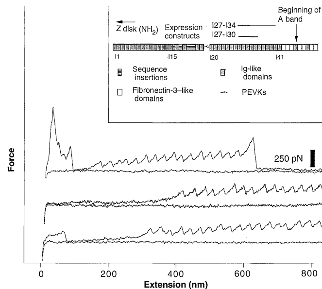
Fig. 1. Force extension curves obtained by stretching titin proteins show periodic features that are consistent with their modular construction. Native titin proteins (10 \mu\text{g}/\text{ml} in PBS) were allowed to adsorb onto a gold surface. Three typical approach and retract cycles are shown. The AFM tip approaches the surface covered with the protein (lower trace), and segments of the adsorbed titin are picked up at random by an AFM tip and then stretched (upper trace). We frequently observed a sawtooth pattern in the retraction curves, with as many as 20 force peaks that varied between 150 and 300 pN and were spaced between 25 and 28 nm. The sawtooth pattern was in most cases preceded by a spacer region of variable length, where the force extension curve was not well defined and varied widely. All experiments were done at room temperature. Titin is a large modular protein composed of 244 repeats of Ig-like and fibronectin-like domains (inset). These domains are 89 to 100 amino acids long. Each domain folds into a seven-stranded beta-barrel. The sawtooth pattern observed while stretching titin segments is consistent with the sequential unfolding of individual titin domains.
