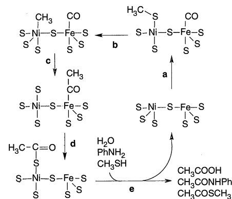
Fig. 2. Notional representation of a hypothetical mechanism of acetic acid formation from CO and CH 3 SH on NiS-FeS. Step a: uptake of CO by an Fe center and of CH 3 SH by an Ni center. Step b: formation of a methyl-Ni center. Step c: migration of methyl to a carbonyl group, forming an Fe-bonded (or Ni-bonded) acetyl group. Step d: migration of acetyl to a sulfido (or sulfhydryl) ligand, forming a thioacetate ligand of Ni (or Fe). Step e: hydrolytic formation of acetic acid. The free valences of the sulfur ligands are either bonded to another metal center or to H (or CH 3 ). Alternatively, in step d the acetyl group may migrate to a CH 3 -S- ligand to form the methylthioester CH 3 -CO-SCH 3 , which subsequently detaches.
