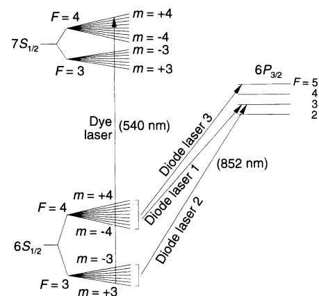
Fig. 1. Partial cesium energy-level diagram including the splitting of S states by the magnetic field. The case of 540-nm light exciting the F = 3, m = 3 level is shown. Diode lasers 1 and 2 optically pump all of the atoms into the (3, 3) level, and laser 3 drives the 6S_{F=4} (F_{\text{det}}) to 6P_{F=5} transition to detect the 7S excitation. PNC is also measured for excitation from the (3, -3) , (4, 4) , and (4, -4) 6S levels. The diode lasers excite different transitions for the latter two cases.
