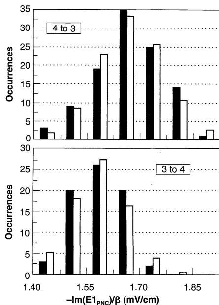
Fig. 3. Histograms of 1.5 hour blocks of PNC results for the 6S_{F=3} to 7S_{F=4} and the 6S_{F=4} to 7S_{F=3} transitions. The solid bars are the data, and the open bars are the theoretical distributions expected for random samples with standard deviations matching the independently measured short-term noise in the data.
