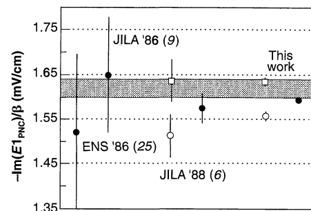
Fig. 4. Historical comparison of cesium PNC results. The squares are values for the 4-3 transition, the open circles are the 3-4 transition, and the solid circles are averages over the hyperfine transitions. The band is the standard-model prediction for the average, including radiative corrections. The \pm 1\sigma width shown is dominated by the uncertainty of the atomic structure.
