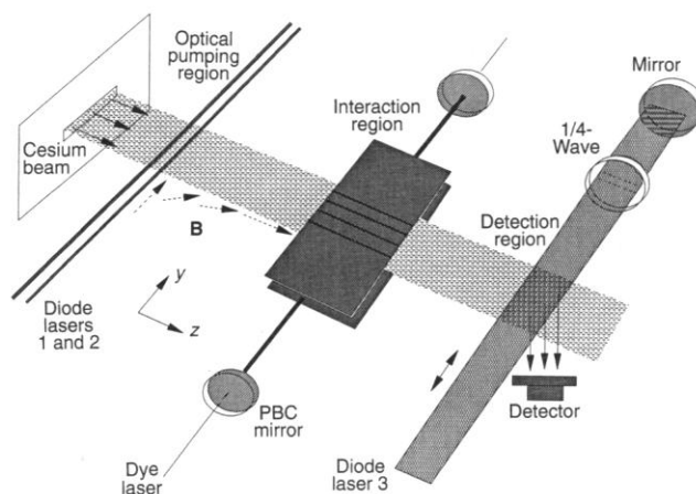
Fig. 2. Schematic of the apparatus. In the interaction region, \mathbf{B} is along the z axis, \mathbf{E} is along the x axis, and the 540-nm dye laser beam defines the y axis.
