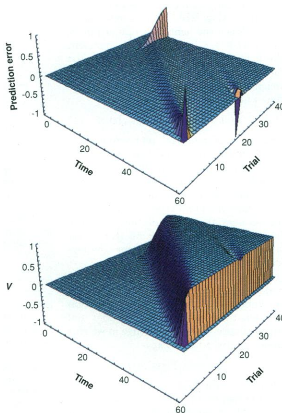
Fig. 3. Development of prediction error signal through training. (Top) Prediction error (changes in dopamine neuron output) as a function of time and trial. On each trial, a sensory cue is presented at time step 10 and time step 20 followed by reward delivery [ r(t) = 1 ] at time step 60. On trial 0, the presentation of the two cues causes no change because the associated weights are initially set to 0. There is, however, a strong positive response (increased firing rate) at the delivery of reward at time step 60. By repeating the pairing of the sensory cues followed in time by reward, the transient response of the model shifts to the time of the earliest sensory cue (time step 10). Failure to deliver the reward during an intermediate trial causes a large negative fluctuation in the model's output. This would be seen in an experiment as a marked decrease in spike output at the time that reward should have been delivered. In this example, the timing of reward delivery is learned well before any response transfers to the earliest sensory cue. (Bottom) The value function V(t) . The weights are all initially set to 0 (trial 0). After the large prediction error occurs on trial 0, the weights begin to grow. Eventually they all saturate to 1 so that the only transient is the unpredicted onset of the first sensory cue. The depression in the surface results from the error trial where the reward was not delivered at the expected time.
