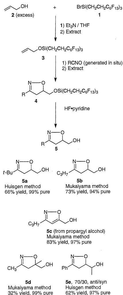
Fig. 2. Nitrile oxide cycloadditions with fluorosubstrate labeled allyl alcohols. The RCNO intermediate is generated as in Fig. 1; here R' would be \text{CH}_2\text{OH} labeled with the fluorosubstrate tag at the oxygen.
