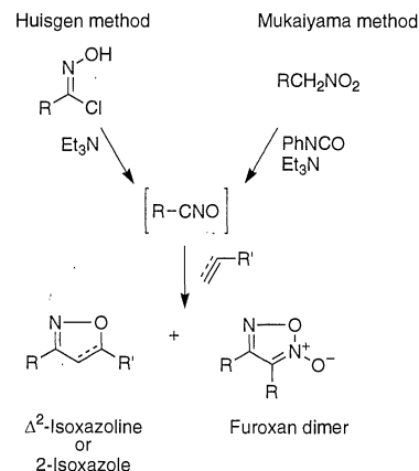
Fig. 1. In situ methods of nitrile oxide generation and cycloaddition.
