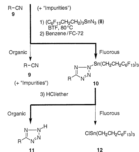
Fig. 4. Combining a fluorine reagent and label. Yields: R = CH 3 , 83%; i -Bu, 87%; PhCH 2 , 77%; p -CH 3 C 6 H 4 , 61%; p -MeOC 6 H 4 , 72%; Ph, 59%; p -NO 2 C 6 H 4 , <10%.
