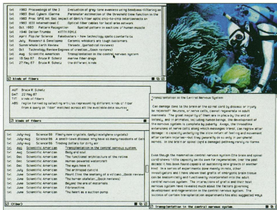
Fig. 2. Telesophy project (1986): a research prototype of the 1980s. The user has issued a broad query (lower left) for "fiber," with the goal of gathering instances of different kinds of fibers. This query was sent out to all the sources within the information space, and the full texts of documents with matching text were returned. After scrolling through the results, the user has located a desired magazine article, which appears from the title to discuss nerve fibers, and zoomed into it. The full text appears in its own window (lower right). A related image also appears (upper right); this picture was linked to the article, and the image displayer was automatically invoked when the link was followed. The window at the upper left illustrates grouping and sharing: It is a region of pointers to located objects, which were copied into the region after being located during a search. The items returned include journal abstracts, magazine articles, and movie reviews. The picture is also an object in the system and thus can be contained in regions, as can the note in the middle left that was entered on the fly. This dynamically created region can be saved and later retrieved by searching on its title (the picture similarly had all text associated with it automatically indexed). All of the pointers in the region are live.
