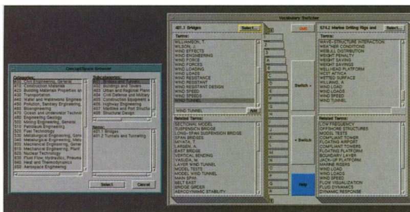
Fig. 4. Interspace project (1996): a research prototype of the 1990s. A sample screen from the vocabulary switching experiment comprising 1000 community repositories with 10 million abstracts across all of science and engineering (computed on 5 years of Compendex and Inspec data using 10 days of supercomputer time on the NCSA HP Convex Exemplar in the spring of 1996). The classification window (left) is the human-indexer categorization showing the subject hierarchy down to "401.1 Bridges." The switching window (right) shows the use of concept spaces for vocabulary switching across community repositories. When a common term occurs across repositories, the system can automatically switch across spaces. The example illustrates a civil engineer who is designing a bridge and is interested in searching ocean engineer literature for similar effects of fluid dynamics on long structures. "Wind Tunnel" is a term common between the repositories for "Bridges" and "Marine Drilling Rigs." The list of related terms on structural stability and fluid dynamics is different because the co-occurrence frequency is different within the two collections. The user can match corresponding terms across spaces, such as "suspension bridges" versus "compliant towers." This match is illustrative of the underlying semantics that suspension bridges have steel cables tethered to prevent swaying in the air, whereas compliant towers are marine rigs with a floating platform tethered to the ocean floor by steel cables that steady the oil drill from swaying in the water.
