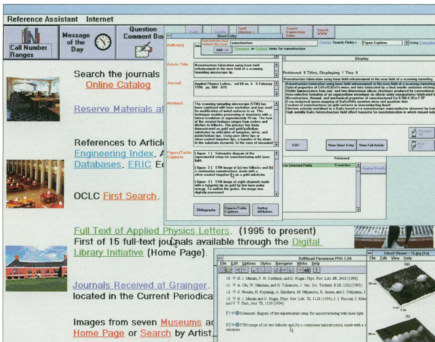
Fig. 3. Illinois DLI project (1996): an experimental testbed of the 1990s. A search query (upper right) uses the structure information in the documents to match “nanostructure” only in figure captions. Matching documents are retrieved across the network, and a summary version is displayed. The full article has been displayed (lower right) in a separate SGML viewer (labeled “SoftQuad Panorama”); the window has been scrolled down to display the
