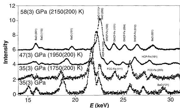
Fig. 2. X-ray data on Fe from different spots. All data are at room T and high P . Temperatures shown in brackets are those at which the sample was heated before quenching. Pressures are determined from the equation of state of BaO (III). Part of the Fe heated to 1750 K ( \pm 200 ) at 35 GPa ( \pm 3 ) transformed to the FCC Fe [reflections (111) and (200)]. At 47 GPa ( \pm 3 ) and 1950 K ( \pm 200 ) appear two exclusive DHCP-Fe reflections (101) and (004). They are accompanied by the (100) and (102) reflections, which could be mixtures of the DHCP- and HCP-Fe. At 58 GPa ( \pm 3 ) and 2150 K ( \pm 200 ), all HCP-Fe, which is in the form of iron powder, may have been converted to the DHCP-Fe. Intensity is in arbitrary units.
