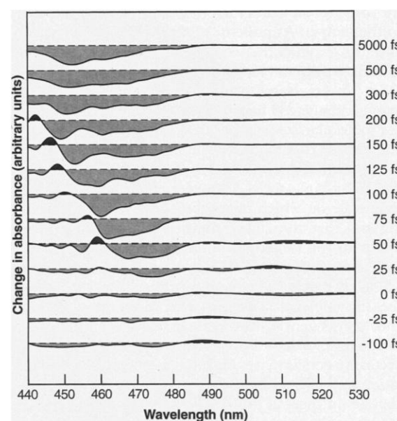
Fig. 2. Femtosecond time-resolved excited-state-ground-state absorption difference spectra for [\text{Ru}(\text{bpy})_3](\text{PF}_6)_2 in \text{CH}_3\text{CN} solution at 298 K (17). The probe pulse gave adequate intensity for probing in the 450- to 530-nm range; below 450 nm, the relative amplitude of the signal dropped due to the vanishing intensity of the probe pulse in this region and the strong ground-state absorbance of the sample. The resulting poor signal-to-noise ratio resulted in some uncertainty in the baseline correction and hence the amplitude of the differential absorption in this portion of the spectrum. The orientation of the probe beam was set at the magic angle ( \sim 55^\circ ) relative to the parallel pump beam to minimize polarization effects. Detection was accomplished with an optical multichannel analyzer (OMA), and wavelength calibration was verified with a HeNe laser. The time delays were effected with an optical delay line. The position of \Delta t = 0 , defined as the maximum of the pump-probe cross correlation, was checked both before and after each full scan, and in no case was the drift over the course of the experiment greater than \sim 5 fs. The dotted line in each spectrum corresponds to \Delta A = 0 , and the inset numbers indicate probe beam delay times from \Delta t = 0 . The data were smoothed with a gaussian smoothing function with a bandwidth of 2 nm; a somewhat broader filter was applied to the data between 470 and 480 nm to compensate for an artifact associated with the OMA.
