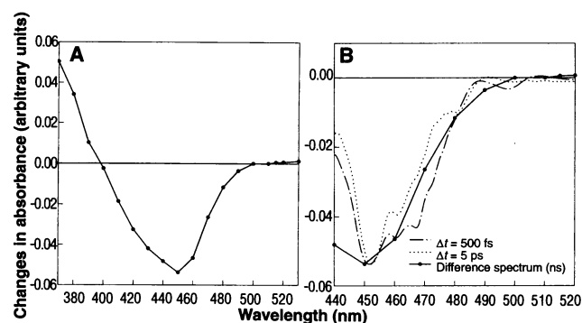
Fig. 3. (A) Excited-state-ground-state absorption difference spectrum of [\text{Ru}(\text{bpy})_3](\text{PF}_6)_2 in \text{CH}_3\text{CN} following nanosecond excitation at 475 nm. The spectrum was obtained point-by-point by plotting the amplitude from a single-exponential fit of the excited-state relaxation data as a function of probe wavelength. The absorptive feature in the ultraviolet ( \lambda_{\text{max}} = 370 nm) is due to ligand-based transitions of the \text{bpy}^- chromophore. The bleach in the region from \sim 400 to 500 nm is a superposition of absorptions associated with the ^3\text{MLCT} state and loss of the strong ground state ^1\text{MLCT} \leftarrow {}^1\text{A}_1 absorption. Extremely weak absorptive features for \lambda > 500 nm are due either to \text{bpy}^- transitions or LMCT transitions of the \text{Ru}^{\text{III}} excited-state chromophore. (B) Overlay of the spectrum of [\text{Ru}(\text{bpy})_3]^{2+} obtained at \Delta t = 500 fs and 5 ps after femtosecond excitation with the absorption difference spectrum of the compound after nanosecond excitation.
