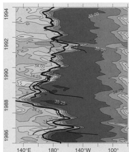
Fig. 5. Longitude-time distribution of 4°N–4°S averaged sea-surface salinity, as simulated by the LODYC model. The trajectories of hypothetical drifters moved by the LODYC-simulated 4°N–4°S averaged zonal current are superimposed (thick solid line). Also shown are examples of several pairs of drifters converging into the main trajectory that closely follows the salinity front (additional lines around 1987, 1989, and 1992).
