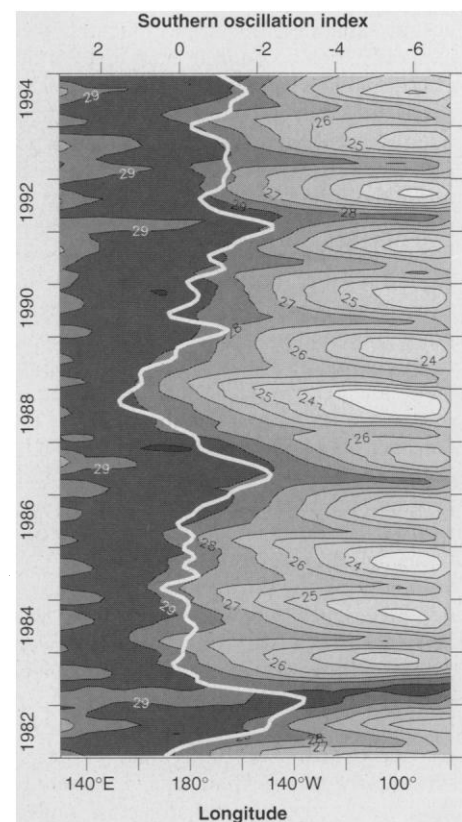
Fig. 1. Longitude-time distribution of the 4^{\circ}\text{N} – 4^{\circ}\text{S} averaged SSTs. The Southern Oscillation Index (SOI, upper scale, normalized difference between the sea level pressure anomalies at Tahiti, French Polynesia, and Darwin, Australia), filtered with a 6-month Hanning filter, is superimposed as a thick white line. The SOI is closely related to SST, surface wind, and atmospheric convection changes in the tropical Pacific. Note the very good phase agreement between the SOI and the El Niño–La Niña migration of the eastern edge of the warm pool.
