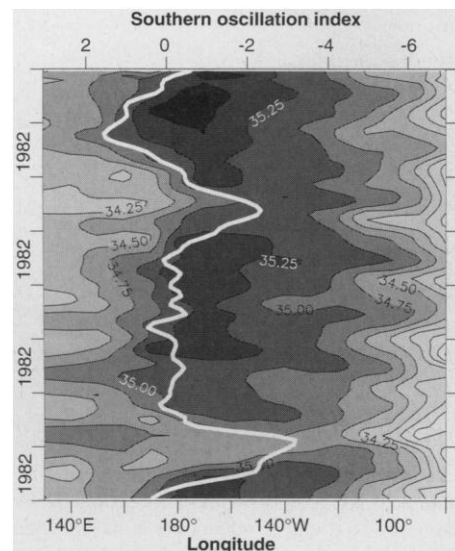
Fig. 4. Longitude-time distribution of 4°N–4°S averaged sea-surface salinity obtained from a ship-of-opportunity network and sparse hydrological data. The SOI is superimposed as a thick white line, as in Fig. 1.
