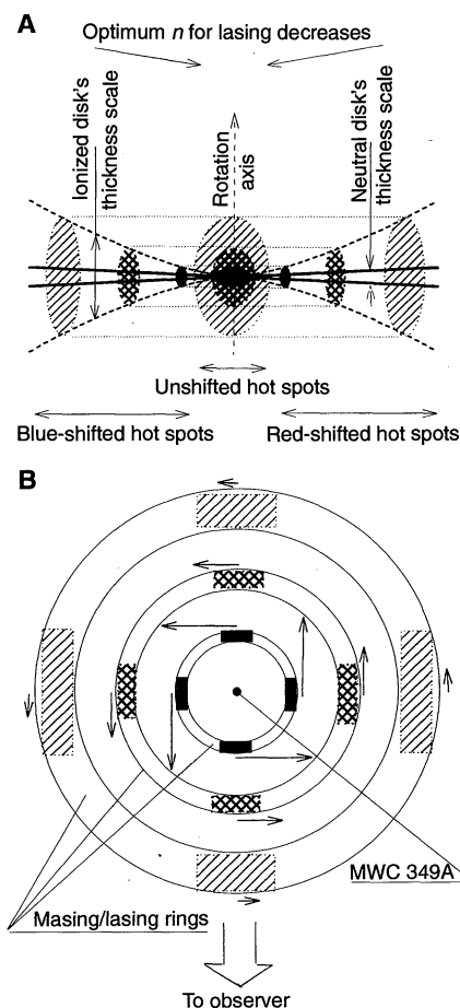
Fig. 3. The putative masing and lasing circumstellar disk in MWC 349A shown (A) edge-on (presumably as we observe it) and (B) face-on. The double-peaked profiles of some infrared spectral lines and the masing millimeter and submillimeter hydrogen lines are ascribed to a Keplerian circumstellar disk seen edge-on (14, 31). According to the model (32) we adopt here, the surface layer of the gas-dust disk surrounding MWC 349A is ionized by the star’s ultraviolet radiation and develops a hydrostatic 10^4\ \text{K} atmosphere inside a critical distance R_g \approx 200\ \text{AU} . Because of decreasing gravitational binding, the atmosphere flares with distance from the star, and beyond R_g it transforms into a stationary bipolar outflow (the outflow is not shown). The electron density in the model atmosphere is \approx 4 \times 10^6\ \text{cm}^{-3} at R_g and is proportional to R^{-3/2} at smaller radii. The velocity vectors in (B) give a rough idea of the Keplerian rotation in the disk. The sense of the rotation is still unknown; it is shown arbitrarily here. The flaring of the disk and the positions and widths of the amplifying rings are not to scale (33). The shaded areas demonstrate the paths of maximal amplification in (B) and the resulting hot spots of maser and laser emission in (A). The increasing density of the shading (from diagonal through hatched to solid) toward the disk’s center illustrates the increasing gas density and, presumably, also the increasing brightness temperature of the masing and lasing hot spots.
