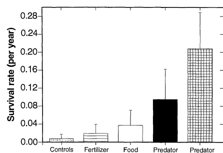
Fig. 4. Annual survival rates for snowshoe hares with radio collars during the decline phase from autumn 1990 to autumn 1992. Ninety-five percent confidence limits are shown. Sample sizes for the estimates are (in order): 278, 206, 197, 246, and 262 hares. Radio collars were placed only on fully grown animals and thus are used to measure adult mortality rates.
