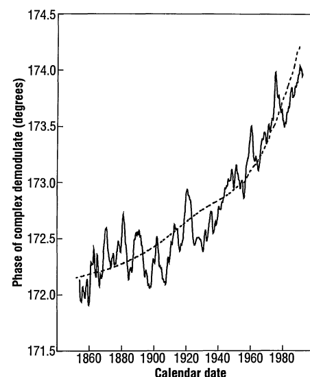
Fig. 12. Phase of the Jones-Wigley Northern Hemisphere land plus marine temperature series, Fig. 5, after a linear offset 50^\circ.256 \cdot (t - 1854) from precession has been added. It is thus an estimate of deviation of the phase from the trend in Fig. 5 that was observed in the early part of the record. The dashed line is a least-squares fit to the phase regressed on the logarithm of atmospheric \text{CO}_2 levels and a constant. For a significance test, see Fig. 13.
