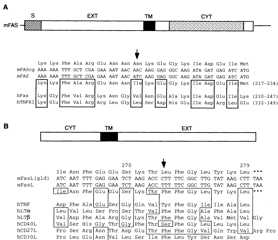
Fig. 2. Mutations in Fas and FasL in lpr and gld mice. (A) A point mutation in the cytoplasmic region of the Fas gene of lpr g mice. The upper panel shows the structure of Fas. S, signal sequence; EXT, extracellular region; TM, transmembrane region; CYT, cytoplasmic region. The Fas death domain, which has similarity with that of TNF-R1, is shown as the shaded area. The lower panel shows the nucleotide sequence and the predicted amino acid sequence of the wild-type (mFAS) and the mutant Fas (mFAScg). The amino acid sequence of the corresponding region of human Fas (hFas) and TNF-R1 (hTNFR1) are also shown. Sets of three identical or homologous amino acid residues at one aligned position are boxed. The arrow indicates the position of the Fas mutation in lpr mice. [Reproduced from (57) with permission from the author and Nature , copyright Macmillan Magazines.] (B) A point mutation in the extracellular region of FasL of gld mice. The upper panel shows the structure of FasL. The lower panel shows the nucleotide and amino acid sequences of the mutant FasL [mFasL(gld)] and wild type (mFasL). The arrow indicates the position of the mutation in FasL of gld mice. Amino acid sequences of the corresponding region of the other members of the TNF family (TNF, LT- \alpha , LT- \beta , CD40L, CD27L, and CD30L) are also shown. The amino acids of favored substitutions in more than four members are boxed. [Reproduced from (22), T. Takahashi et al. , with permission from the author and Cell , copyright Cell Press.]
