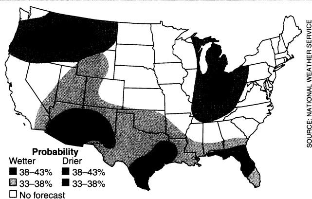
Chances of precipitation. El Niño may bring extra rain to the Gulf Coast and less moisture than normal to the north.
