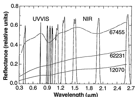
Fig. 3. Bandpasses of Clementine filters for the UVVIS and NIR cameras superimposed on reflectance spectra of lunar samples. In addition to these 10 filters, the UVVIS camera contained a broadband visible filter, and the NIR camera contained an additional filter centered near 2.8 \mu\text{m} . Sample 67455 is a feldspathic rock powder with low-calcium pyroxene from Apollo 16; sample 62231, an Apollo 16 soil, is also feldspathic, and the Apollo 12 soil (12070) is basaltic.
