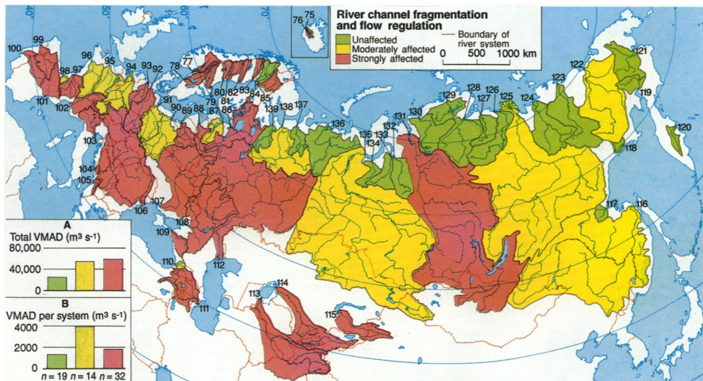
Fig. 2. Impact by river channel fragmentation and flow regulation on the 65 LRSs ( \text{VMAD} \geq 350 \text{ m}^3 \text{ s}^{-1} ) of Europe and the republics of the former Soviet Union. River systems are treated as units and are represented on the map by their catchments. White areas indicate land not covered by LRSs and land
