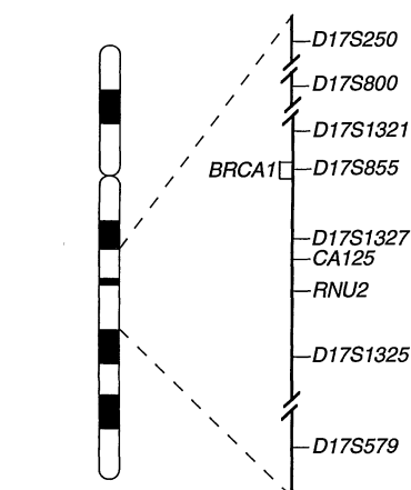
Fig. 1. Schematic map of human chromosome 17. The pertinent region containing BRCA1 is expanded to indicate the relative positions of two previously identified genes, CA125 (34) and RNU2 (45). D17S855 is located within BRCA1 .
