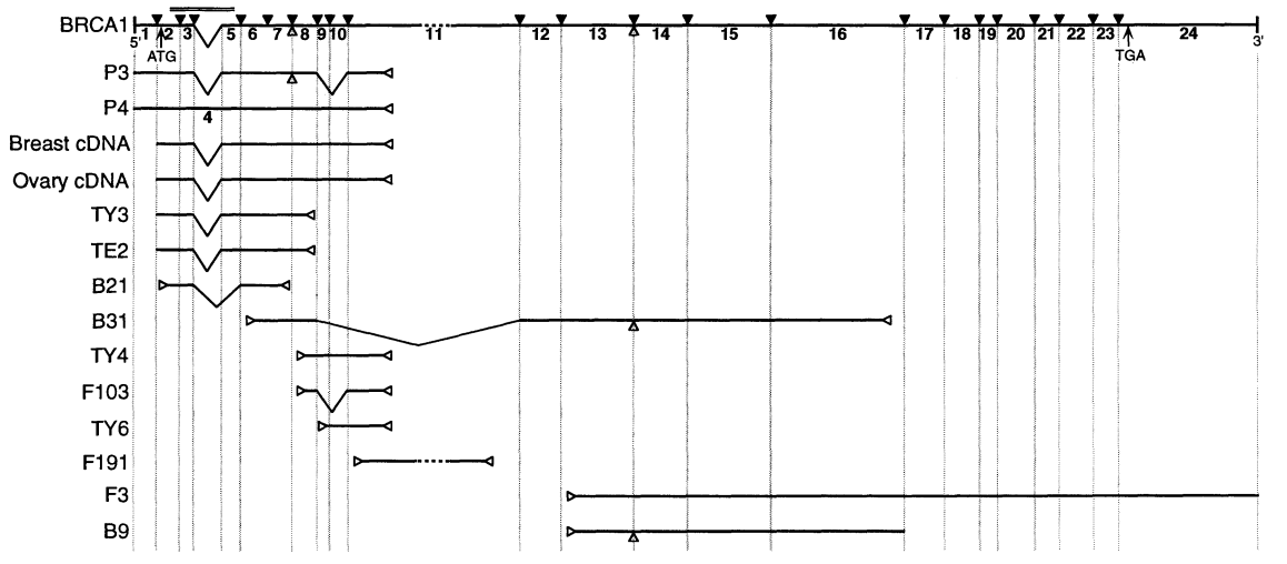
Fig. 3. Diagram of BRCA1 mRNA, showing the locations of introns and the variants of BRCA1 mRNA produced by alternative splicing. The top cDNA ( BRCA1 ) is the composite used to generate the protein sequence in Fig. 2. Intron locations are shown by filled triangles, and the exons are numbered below the composite cDNA. Alternative mRNAs identified as cDNA clones or in hybrid-selection experiments are shown below the composite. The start codon (ATG) and stop codon (TGA) are indicated. The zinc finger region is denoted noted by a double line. "V" lines connecting exons indicate the absence of internal exons. All exons are drawn proportionally except exon 11 (indicated with a dotted line). Upward-pointing unfilled triangles show the position of a single codon (CAG) found at the start of exons 8 and 14 in some cDNAs. Leftward- and rightward-pointing unfilled triangles represent partial exons in some cDNAs. P3 and P4 are cDNA clones isolated from a placental cDNA library;
