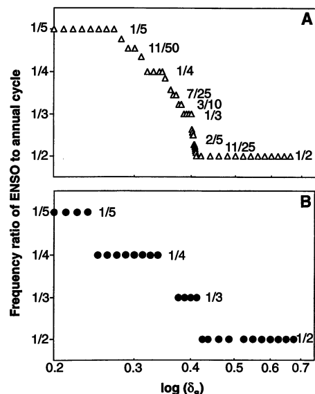
Fig. 1. Frequency ratio of the model El Niño oscillation to the annual cycle, as a function of a parameter, \delta_s , that affects the inherent ENSO period. Another parameter, the coupling coefficient, \mu , is changed to keep the El Niño cycle below its transition to chaos. Nonlinear frequency locking to the annual cycle creates a staircase of discrete steps at rational values of the frequency ratio. For instance, for a frequency ratio 1/4, the ENSO period is exactly 4 years, while for 3/10, a sequence of three El Niño cycles repeats every 10 years. (A) The approximate devil's staircase, slightly above the primary Hopf bifurcation where the ENSO mode goes unstable. All points shown correspond to rational frequency ratios (some labeled). (B) Frequency-locked solutions for slightly larger (by about 10%) values of \mu , showing the rapid widening of the integer-period steps.
