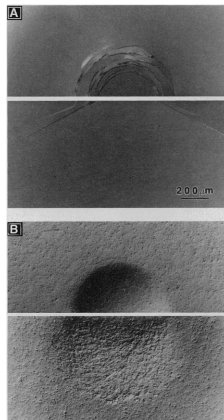
Fig. 4. Half-surface (top) and section (bottom) views of Hertzian contact damage in glass-ceramic, from a tungsten carbide sphere of radius r = 3.18 \text{ mm} at load P = 1000 \text{ N} . (A) Base glass form showing well-defined cone crack (stress p_0 = 2.88 \text{ GPa} ); (B) partially crystallized form showing distributed subsurface damage (stress p_0 = 1.87 \text{ GPa} ).
