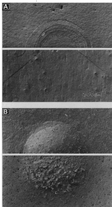
Fig. 2. Half-surface (top) and section (bottom) views of Hertzian contact damage in silicon carbide, from a tungsten carbide sphere of radius r = 3.18 \text{ mm} at load P = 2000 \text{ N} . (A) Homogeneous fine-grain form showing well-defined cone crack (stress p_0 = 7.44 \text{ GPa} ); (B) heterogeneous coarse-grain form showing distributed subsurface damage (stress p_0 = 7.20 \text{ GPa} ).
