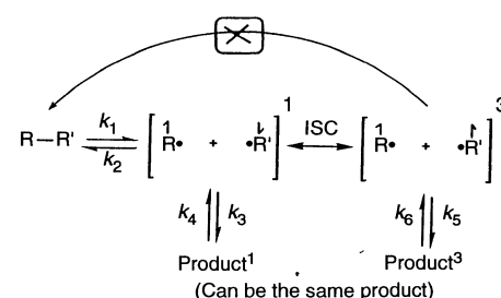
Fig. 1. Effect of a magnetic field on radical pair recombination rates in a chemical reaction.
