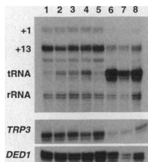
Fig. 3. Transcriptional analysis of strains that carry temperature-sensitive TBP alleles. The TBP derivatives were as follows (28): lane 1, E129S; lane 2, R137W; lane 3, F152E; lane 4, R220K; lane 5, Y231V; lane 6, F237R; lane 7, A217P; and lane 8, wild-type. RNAs were prepared from cells grown at the restrictive temperature (37°C) for 1 hour and subjected to nuclease S1 analysis as described (2). Equal amounts of RNA (determined by absorbance at 260 nm) were hybridized to completion with a 10- to 100-fold excess of oligonucleotide probes complementary to TRP3 , DED1 , and HIS3 +1 and +13 transcripts, the junction of the 25S rRNA and nontranscribed spacer region, and the intron of the Ile tRNA. Because the half lives of these RNA species are short, the signal at any given time reflects transcription initiation, not accumulated RNA levels (2).
