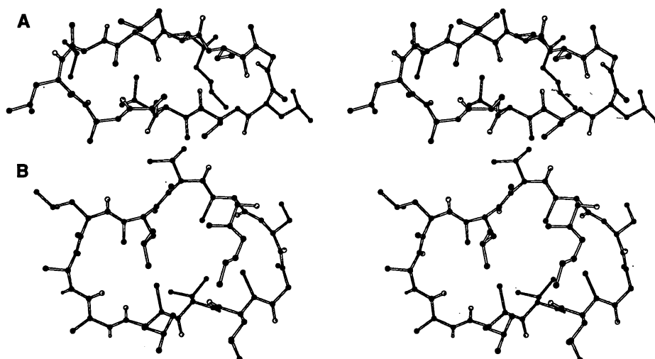
Fig. 1. (A) Stereodiamgram of the unbound conformation of CsA in the solid state. (B) Stereodiamgram of the cyclophilin A-bound conformation of CsA.
