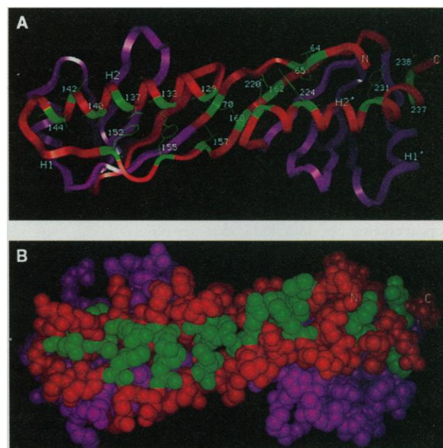
Fig. 4. Mapping the Pol III-specific mutations onto the structure of A. thaliana TBP. The Saccharomyces cerevisiae and A. thaliana TBPs are 85% identical, and therefore the structures are expected to be highly related. (A) Ribbon diagram showing residues not mutated in this study (purple), residues that were mutated but did not yield a Pol III-specific phenotype (red), and residues that did mutate to a Pol III-specific phenotype (green). In this view, the protein has been rotated around the x axis from the standard view (27) such that helices H2 and H2' are facing forward and the concave surface of the protein and stirrups face into the page. (B) Space-filling model of the identical view of TBP. In the same color scheme, the atoms are shown as solid spheres of radius equal to the van der Waals radius.
