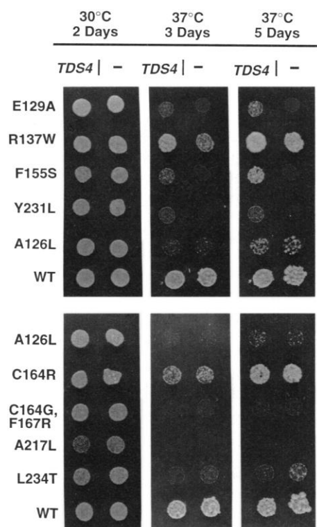
Fig. 5. Suppression of the growth defect of various TBP strains by overexpression of the TFIIIB component Tds4. The TDS4 gene (19) was cloned into an ADE2 2 \mu vector. The resulting molecule and the parental vector were introduced into temperature-sensitive strains that carried the indicated TBP alleles. Approximately 10^5 cells were spotted onto synthetic plates lacking adenine, and these were grown at 30°C or 37°C for the indicated times. The E129A, R137W, F155S, and Y231L mutants (28) are Pol III-specific TBP derivatives; the others are not. Only a subset of strains subjected to this assay are shown; these were chosen to indicate the range of growth and suppression phenotypes. WT, wild type.
