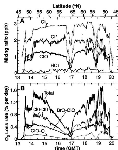
Fig. 1. Observations and reconstructions for 20 January 1992. (A) Observed mixing ratios of ClO and HCl, inferred mixing ratios for Cl* and Cl 2 , and (B) the 24-hour mean loss rates for ozone, computed using Eq. 4 and Cl* shown in (A). The total recombination rate and contributions from the ClO-ClO, BrO-ClO, and ClO-O catalytic cycles (reactions 1, 2, and 3) are shown. All measurements taken along the ER-2 flight track, plotted against universal time (GMT). Corresponding latitudes are indicated at the top of the figure.
