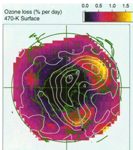
Fig. 4. Distribution of the 24-hour mean loss rate for O 3 (percent per day) in the north polar vortex for the 470 ± 10 K isentrope, derived with global fields of PV and the relation between Cl* and PV shown in Fig. 3, as described in the text. Contours of PV (in units of 10 -5 K m 2 kg -1 s -1 ) and the flight track of the ER-2 (black line, with circle denoting Bangor, Maine) are shown. Latitude circles 60° and 30°N and a map of the continents are denoted by green lines.
