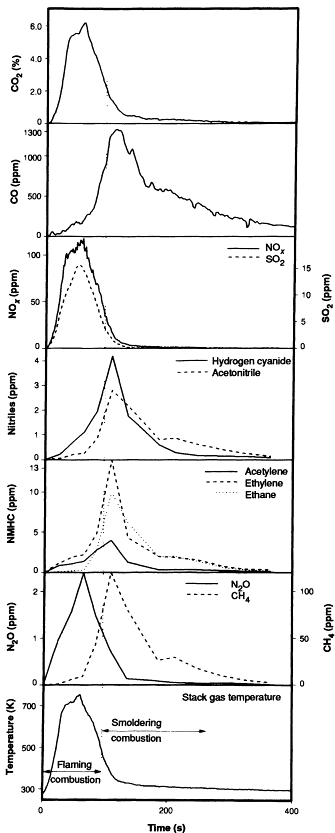
Fig. 1. Concentrations of \text{CO}_2 , \text{CO} , and various other gases in the smoke from an experimental fire of Trachypogon grass from Venezuela as a function of time and the stack gas temperature. The dotted line separates the flaming phase from the smoldering phase. The flaming stage in this fire lasted for about 96 s. Concentrations are in percent by volume for \text{CO}_2 , in volume mixing ratios (ppm) for the other species (1% = 10,000 ppm). Note that \text{CO}_2 , \text{NO}_x , \text{SO}_2 , and \text{N}_2\text{O} are mainly emitted in the flaming phase and the other gases in the smoldering phase; NMHC, nonmethane hydrocarbons.
