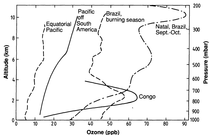
Fig. 2. Vertical profiles of O_3 in the tropical troposphere. The profile over the equatorial Pacific shows no influence from biomass burning), whereas the profile over the Pacific off South America suggests O_3 enhancement due to long-range transport from the tropical continents (47). The O_3 profiles over Brazil (29) and the Congo (51) show high O_3 concentrations at altitudes between 1 and 4 km due to photochemical production in biomass burning plumes. At higher altitudes, O_3 concentrations are also substantially enhanced, possibly also because of O_3 production by reactions in the effluents of biomass burning (48). [Adapted from (47) with permission of the author]
