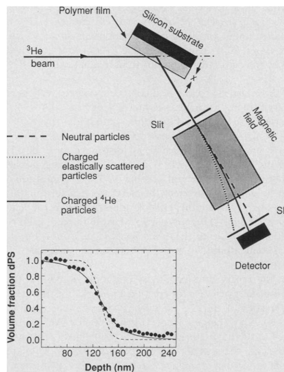
Fig. 2. Schematic illustration of the nuclear reaction analysis experiment (24). The ^3\text{He} beam incident on the polymer bilayer undergoes the reaction ^3\text{He} + ^2\text{H} \rightarrow ^4\text{He} + ^1\text{H} + 18.35 \text{ MeV}
