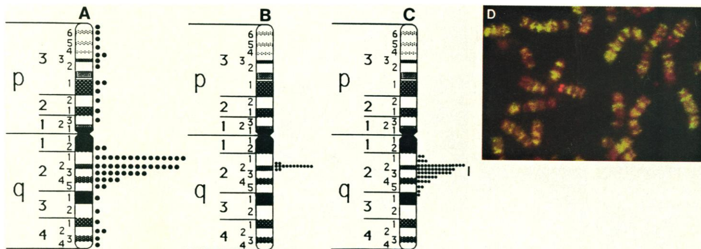
Fig. 1. Comparison of Blast-1 gene localization methods. (A) Autoradiographic detection on G-banded chromosomes with a ^3\text{H} -labeled cDNA probe localized this gene to 1q21–1q23, as reported (11). [Reprinted from (11) with permission, ©1989 Rockefeller University Press.] (B) Fluorescence detection on G-banded chromosomes (15 determinations). Metaphase figures were Giemsa-trypsin-banded, photographed, and rephotographed after hybridization with Blast-1 genomic phage probes. Total chromosome morphology was visible with fluorescein, allowing precise alignment on a grid of the Giemsa-stained and fluorescein-stained chromosomes; centromeres and telomeres were used as reference points. Although trypsinization weakens hybridization signal slightly, this 20-kb target was still clearly detectable. Dots smaller than those in (A) were used to accommodate more precise placement of fluorescent signals. Despite varying chromosome condensation, this gene consistently localized to the interface of 1q21 and 1q22. (C) Fluorescent detection on unbanded chromosomes (55 determinations). Signals were localized by measurement. To correct for chromosome condensation, each data point was expressed as the ratio of the distance from telomere to signal to the total chromosome length. Measurements were made from enlarged photographs by two investigators with essentially
