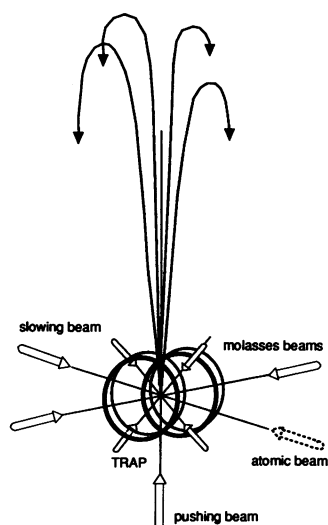
Falling atoms. A laser pushes the atoms up out of the trap, creating a "fountain."
